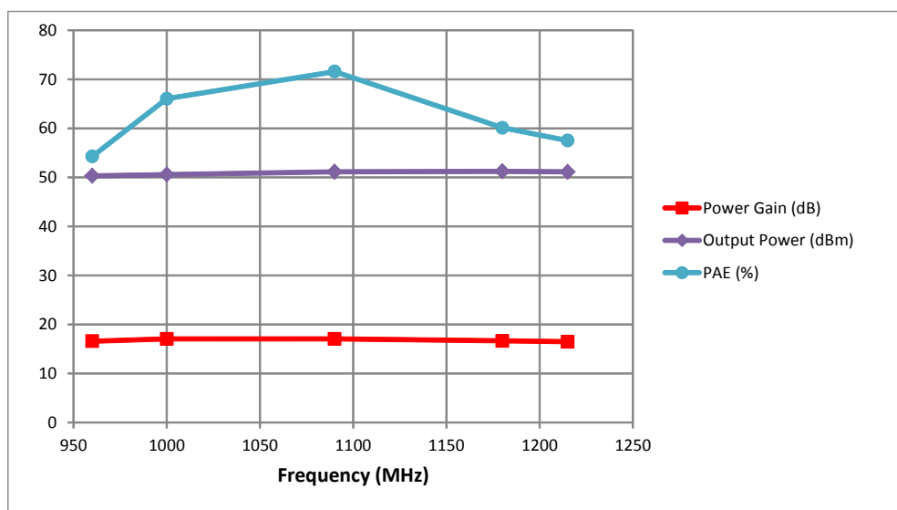
Large-signal Performance Summary of the PA
