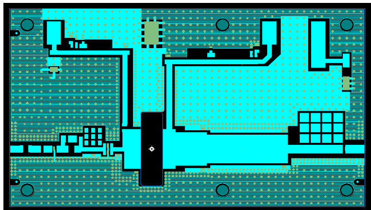
PCB Layout
