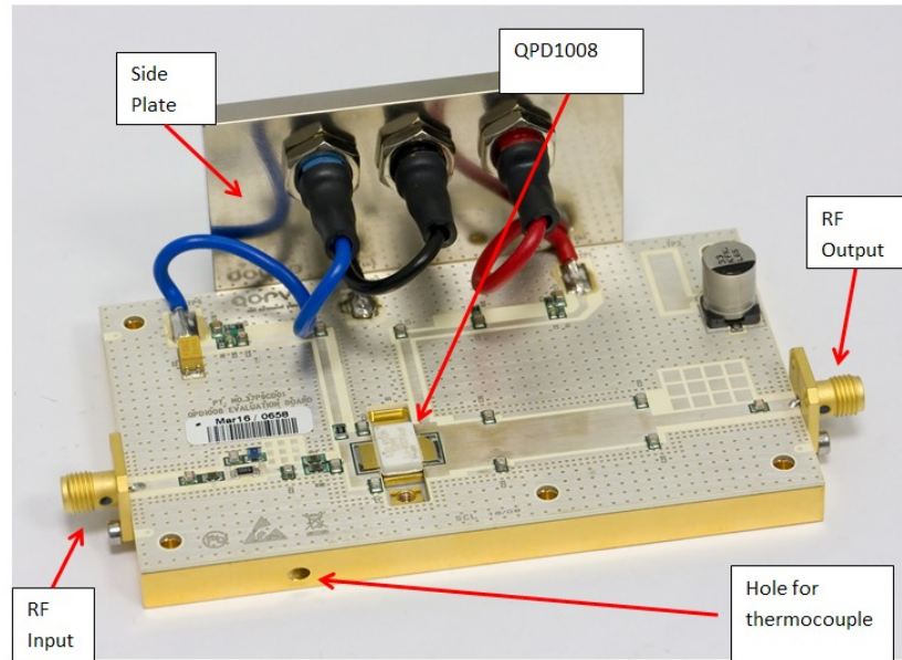
Full Amplifier Assembly
