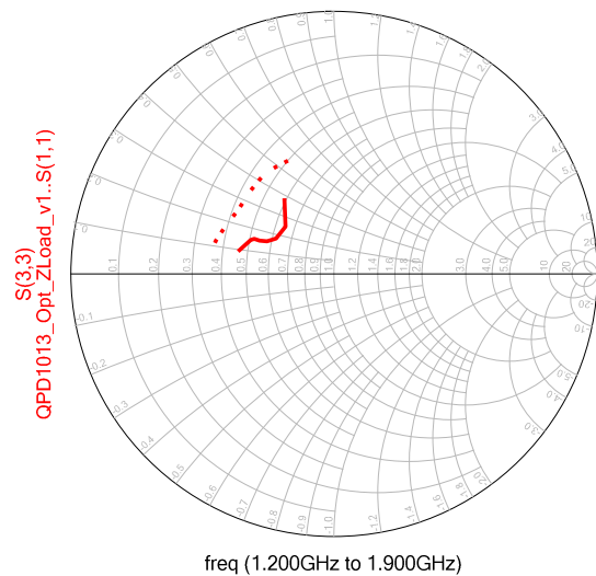
Figure 4: Target (dotted) to simulated (solid) load impedance, 10 Ω chart
