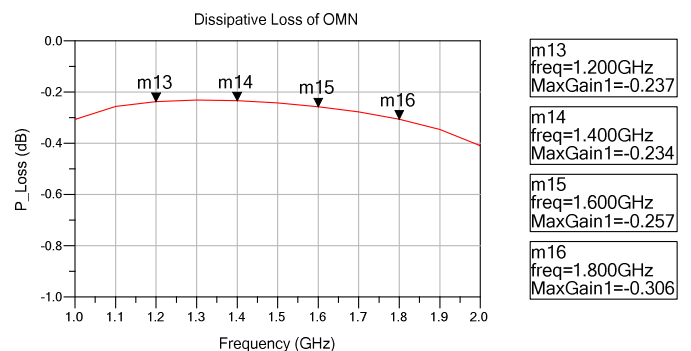
Figure 5: Simulated insertion loss of output network
